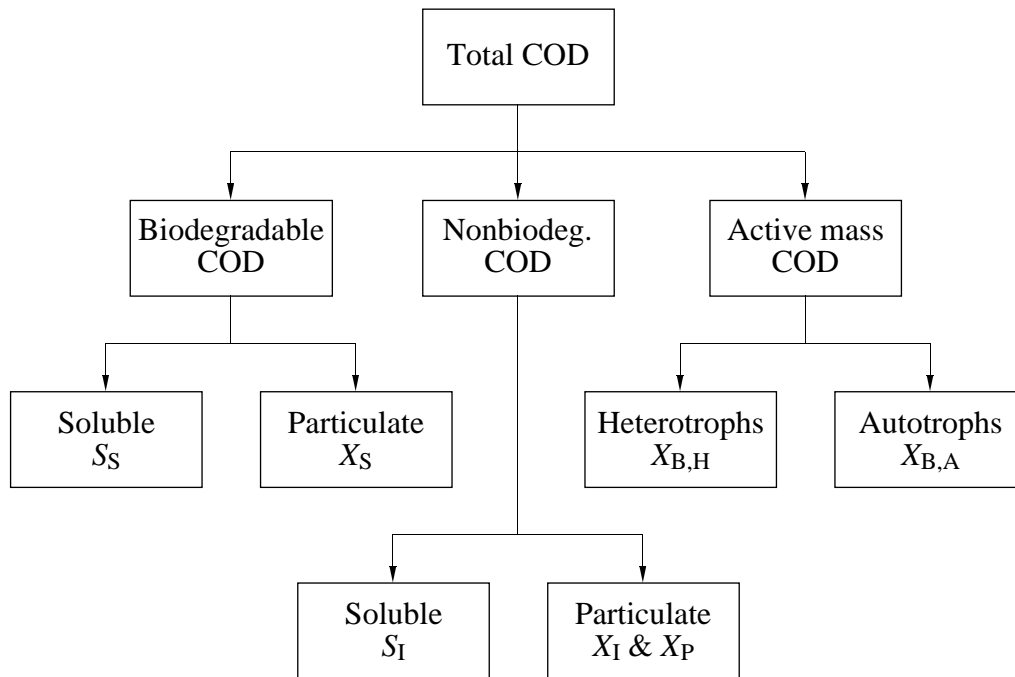
Figure 1 Wastewater characterization for carbonaceous components.
