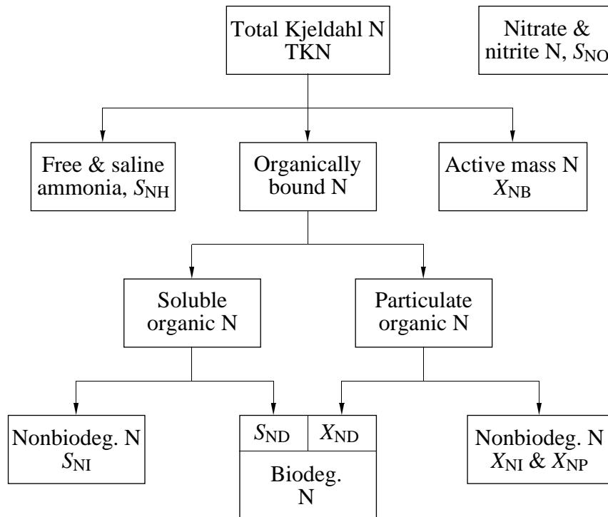
Figure 2 Wastewater characterization for nitrogenous components.
