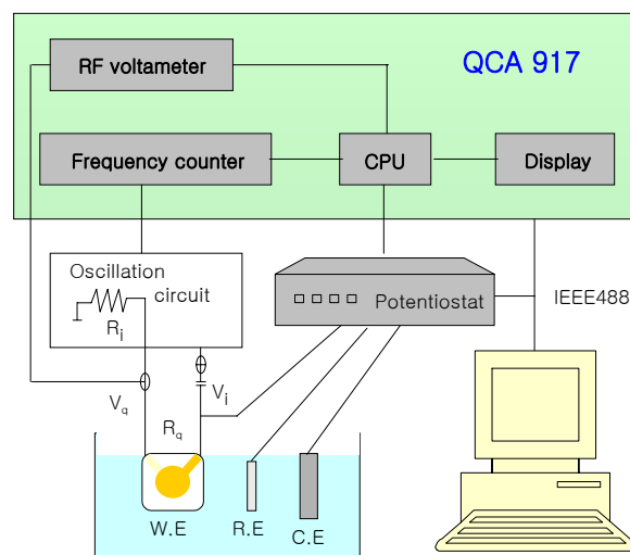
Fig. 2. Schematic diagram of electrochemical experiment for QCA 917.
