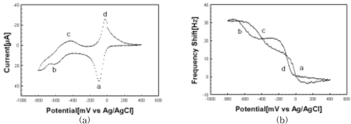
Fig. 4. Cyclic Voltamograms(a) and frequency behavior of QCM modified with Viologen SA monolayer. 0.1mol/l NaClO 4 solution.
