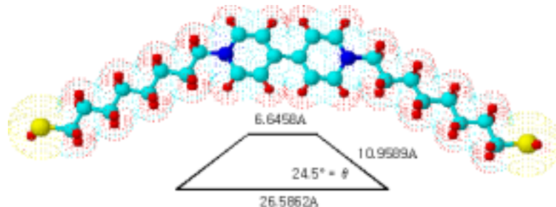
Fig. 1. The chemical structure of Viologen used in this study.
