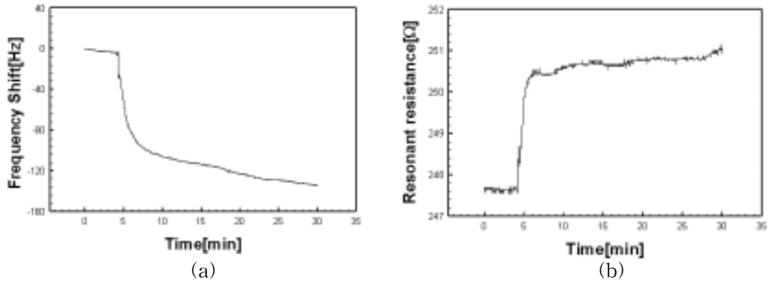
Fig. 3. The time dependence frequency(a) and resonant resistance(b) shift during self assembly process of Viologen
