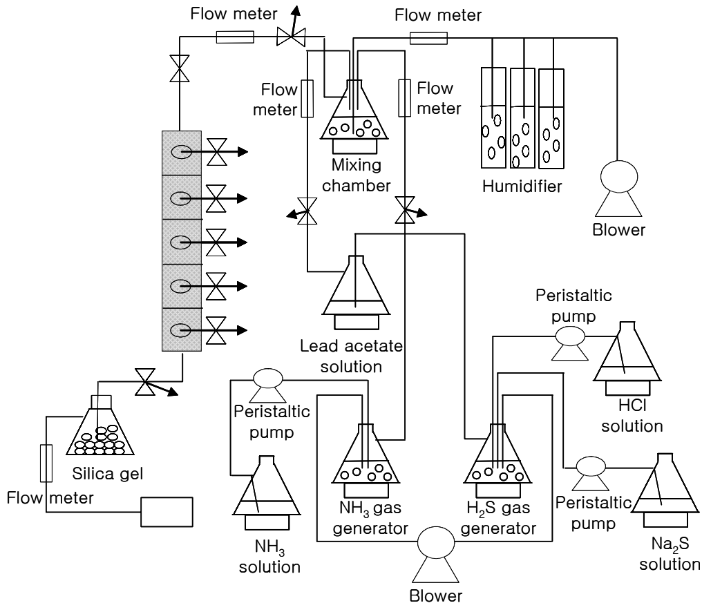
Fig. 1. Schematic diagram of semi-pilot scaled biofilter-system
