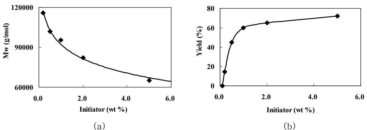
Figure 2. Variation of Molecular Weight (a) and Yield (b) of PVAc upon the Amount of Initiator at 345 bar and 338.15 K for 10 hours.
