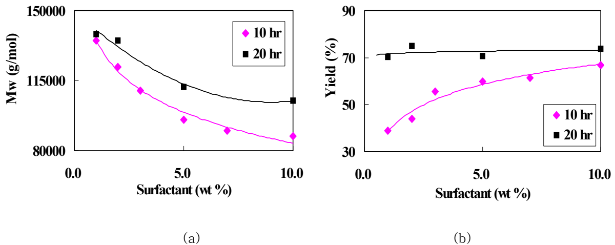
Figure 3. Variation of Molecular Weight (a) and Yield (b) of PVAc upon the Amount of Surfactant for 2 Different Reaction Time at 345 bar and 338.15 K.
