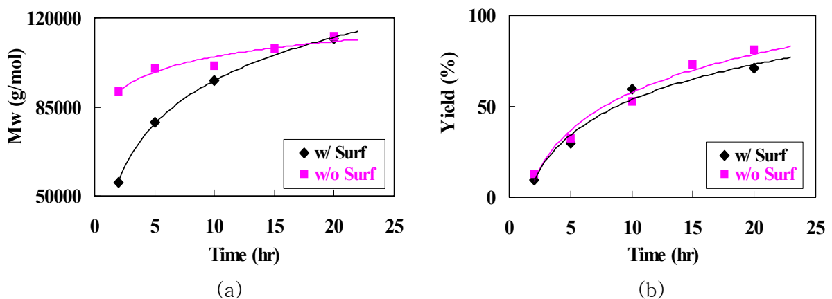
Figure 4. Variation of Molecular Weight (a) and Yield (b) of PVAc upon Reaction Time w/ and w/o Surfactant at 345 bar, 338.15 K.
